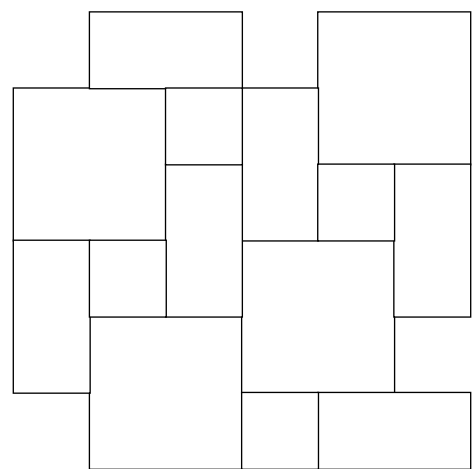
ROMAN PATTERN - 8 SF (4) 12X12, (6) 6X12, (4) 6X6
