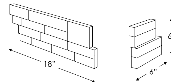
DOGEAR CORNER
