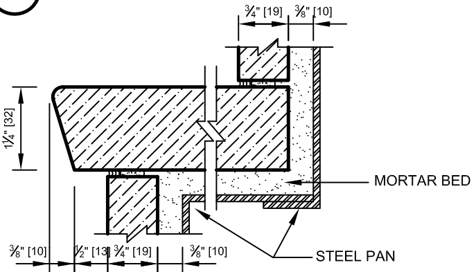
3 STEP DETAIL ON METAL PAN
