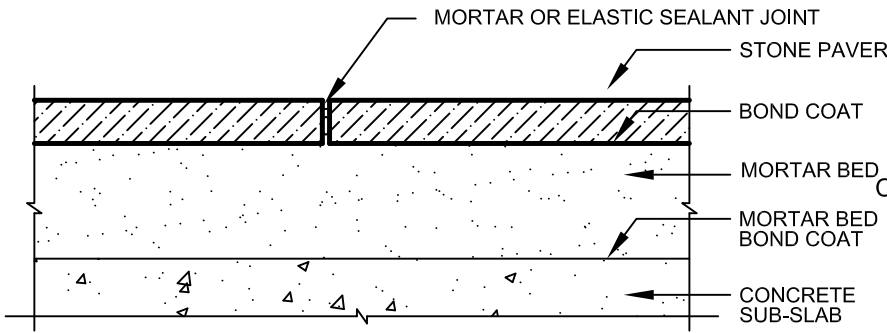
1 MORTAR BED WITH BOND COAT
