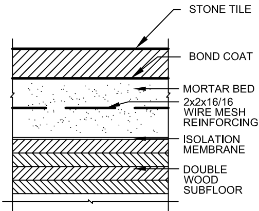
3 STONE TILE SET IN REINFORCED MORTAR BED OVER WOOD FRAME
