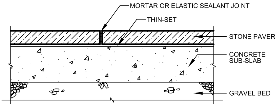
2 MORTAR BED WITH THINSET
