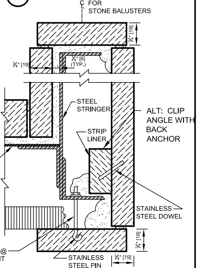
5 STEP DETAIL ON METAL PAN
