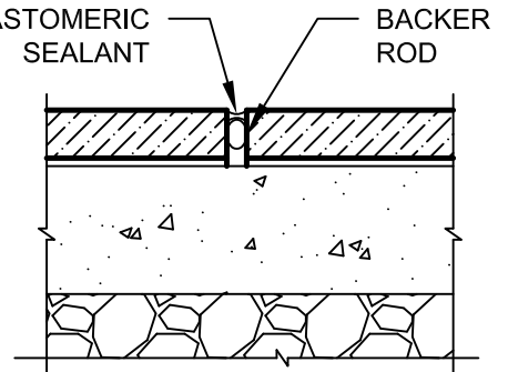
2A MOVEMENT JOINT
