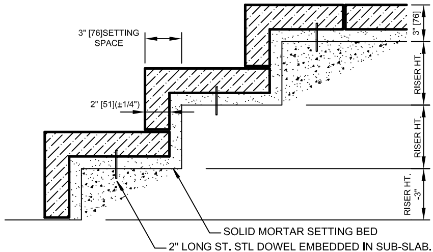
6 HOOKED STEP DETAIL
