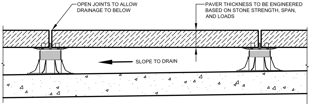
2 PEDESTAL SUPPORTED STONE PAVERS Scale: 1/2" = 1'-0"
