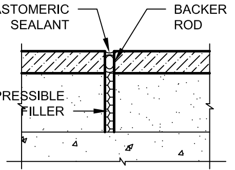
1A MOVEMENT JOINT
