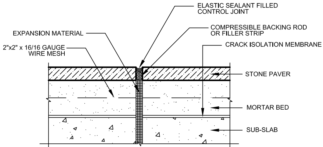
3 FULL MORTAR BED WITH MEMBRANE AND EXPANSION JOINT
