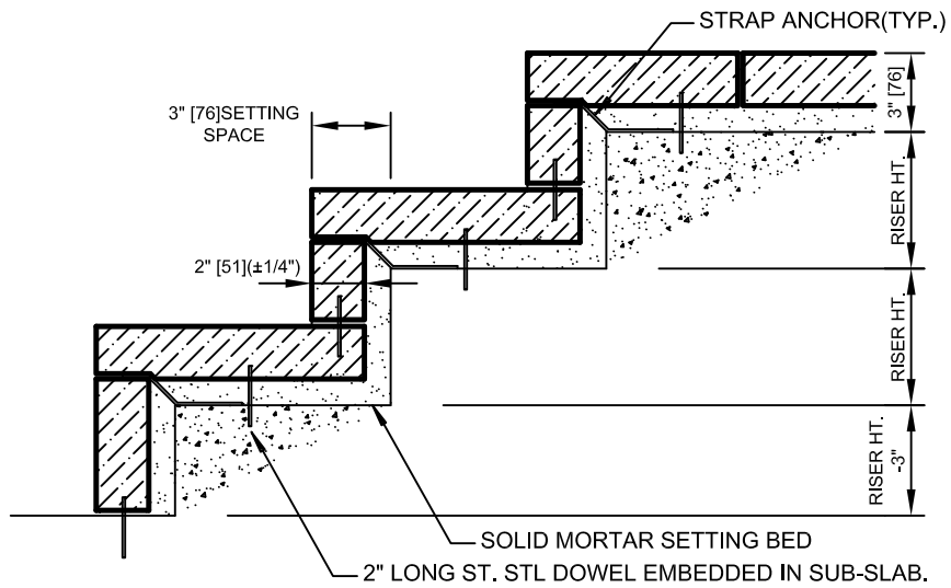
5 VENEERED STEP DETAIL
